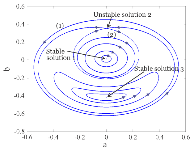
Figure 8. Phase plane of a and b when \Omega R\sqrt{\rho/\mu} = 2.4 , \rho R/\mu H = 0.1 , \varepsilon \Phi_{dc}^2/\mu H^2 = 0.1 and \Phi_{ac}/\Phi_{dc} = 0.1 .
