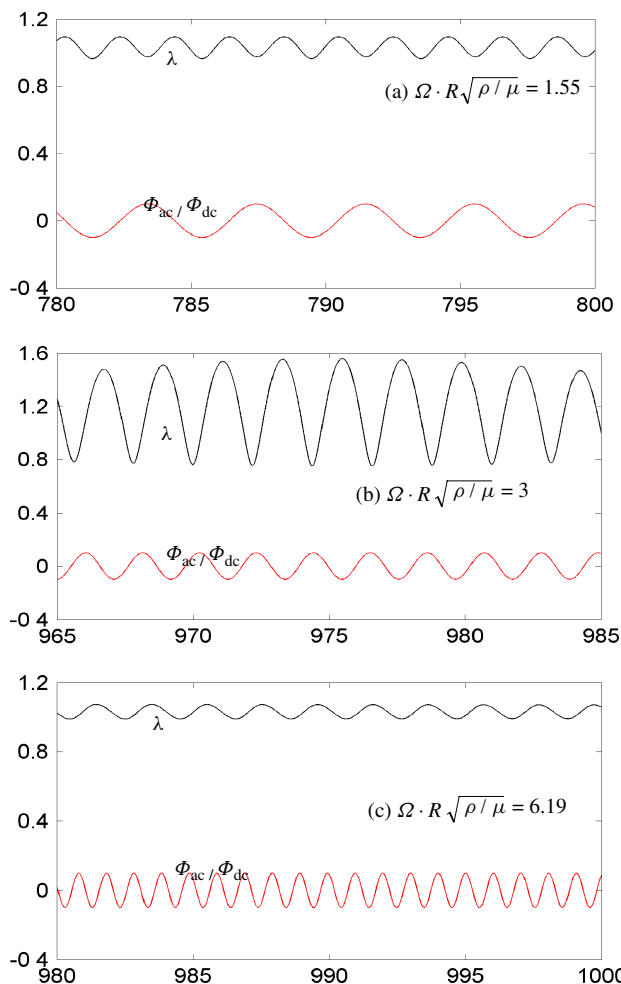
Figure 6. Superharmonic, harmonic and subharmonic responses ( \rho R/\mu H = 0.1 , \varepsilon \Phi_{dc}^2/\mu H^2 = 0.1 and \Phi_{ac}/\Phi_{dc} = 0.1 ).
