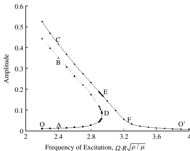
Figure 7. Steady-state solutions when \rho R/\mu H = 0.1 , \varepsilon \Phi_{dc}^2/\mu H^2 = 0.1 and \Phi_{ac}/\Phi_{dc} = 0.1 .
